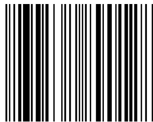
EAN-13
